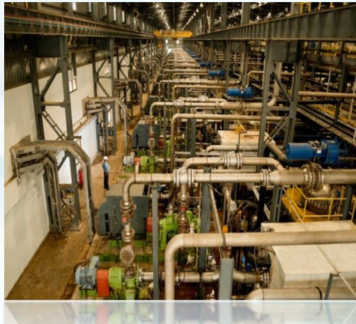
100 MLD Nemmeli, Chennai
